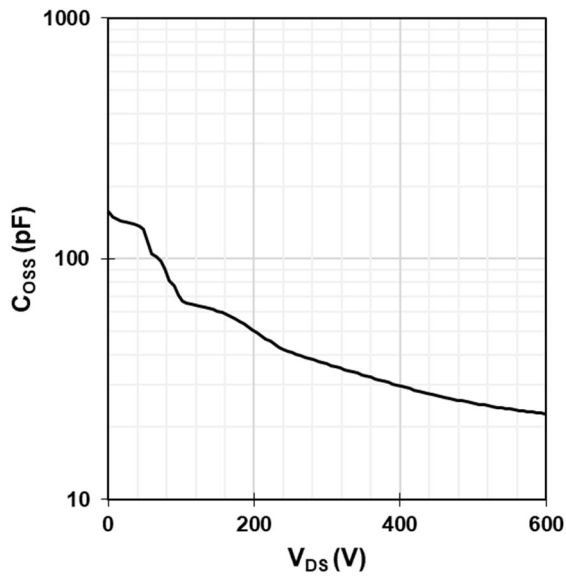
Figure 5 Typ. output capacitance
