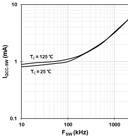
Figure 7 VCC operating current ( I_{QCC-SW} ) vs. F_{SW}
